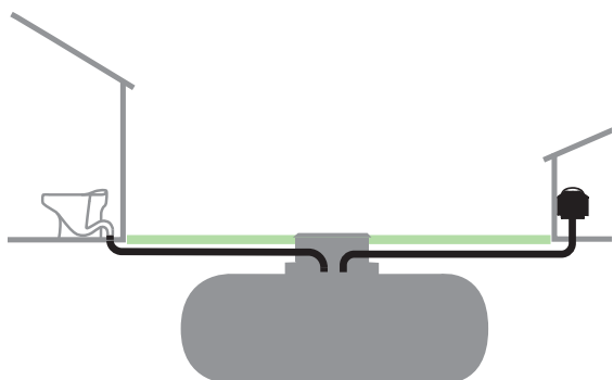
1 WC till 3000 L tank. EcoVacs standardpaket BASE.
